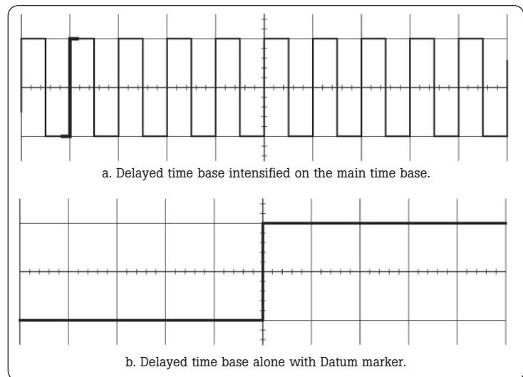
Fig. 1.12 Adjusting the delayed time base to the first Datum marker.
