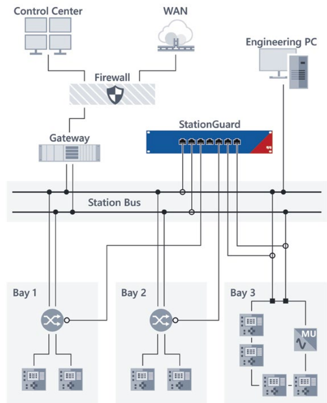
Figure 2: Structure of a substation with connected IDS.
